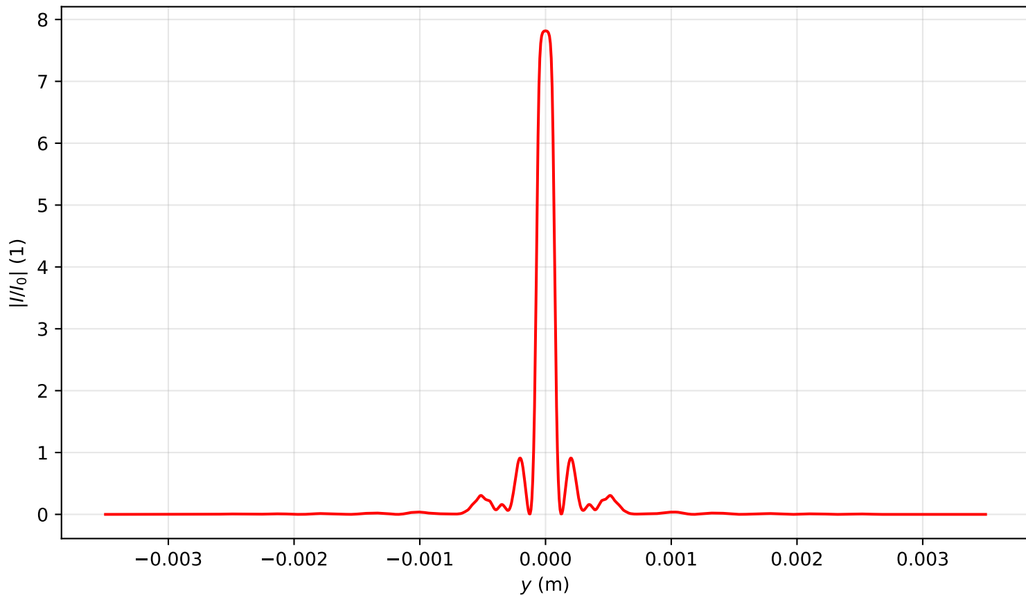
Intensity profile I(x=0, y, z=0.318)/I_0 , \text{Pin}=9.0\text{Pcr} , artificial time
